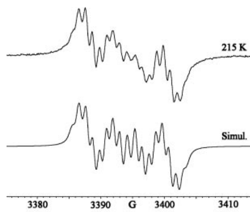
Figure 1. 9-GHz EPR spectrum obtained on treatment of 1a with LDA in THF at 215 K with UV photolysis. Lower panel: computer simulation.
